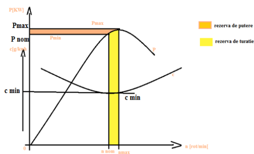
Fig. 4. External feature of the thermal engine Source: authors.
