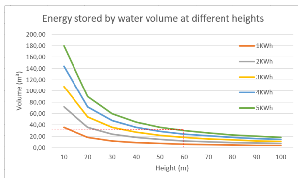
Fig. 4. Water volume needed for storing different energy levels depending on height Source: own processing.
