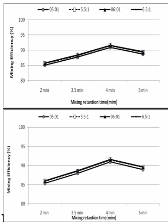
Fig.6. Effect pre-conditioner retention time on mixing Efficiency using rollers teeth width of 10 mm.
