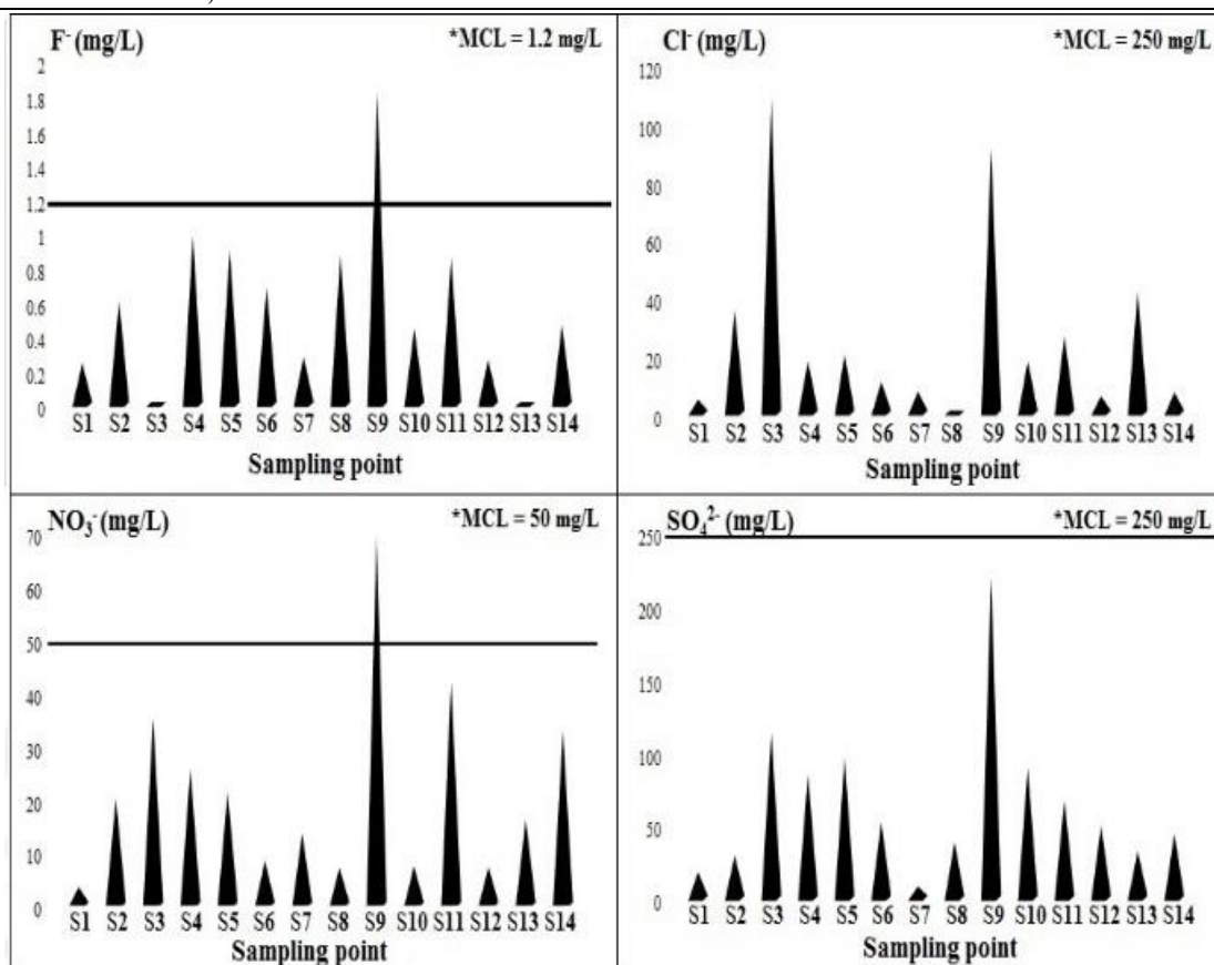
Fig. 4. The level of major dissolved anions
