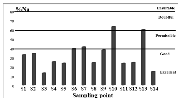
Fig. 6. The percent of Na for the groundwater samples
