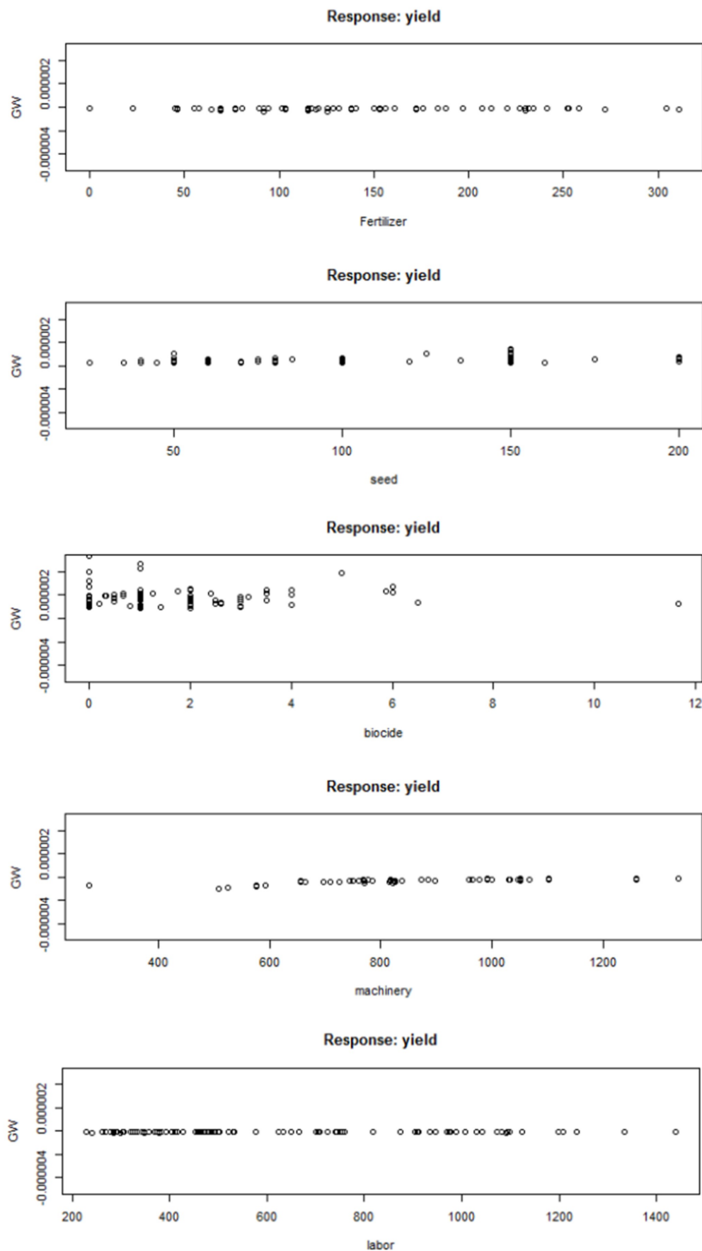
Fig. 2. Plots of generalized weights with respect to each covariate.
