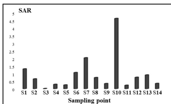
Fig. 5. The level of sodium adsorption ratio (SAR) for the groundwater samples
