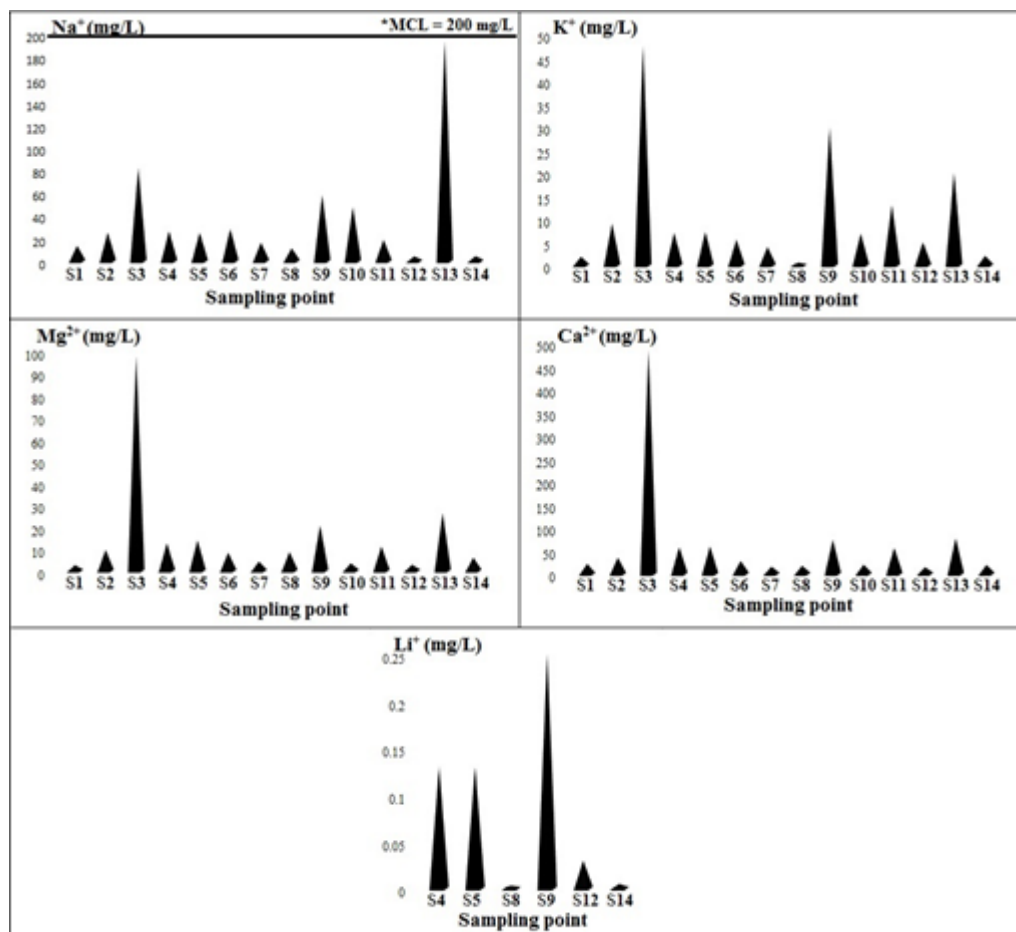
Fig. 3. The level of major dissolved cations
